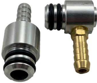
1 x Straight Union 1 x Right Angle Union
